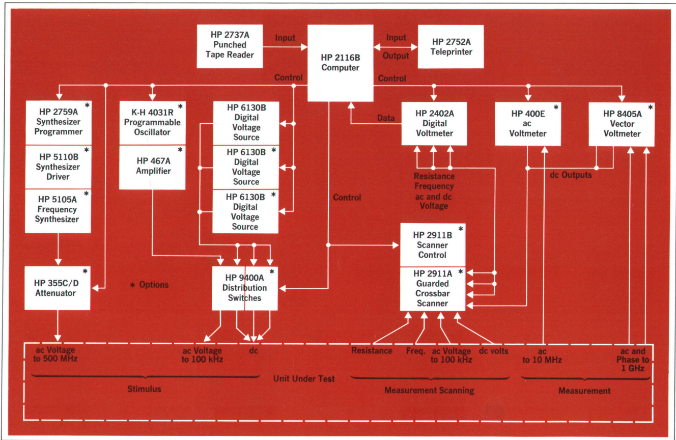
Fig. 2. Model 9500A is a good example of the use of standard instruments and computer interfaces to make a system adaptable and expandable. Many automatic test systems are now being made this way.
