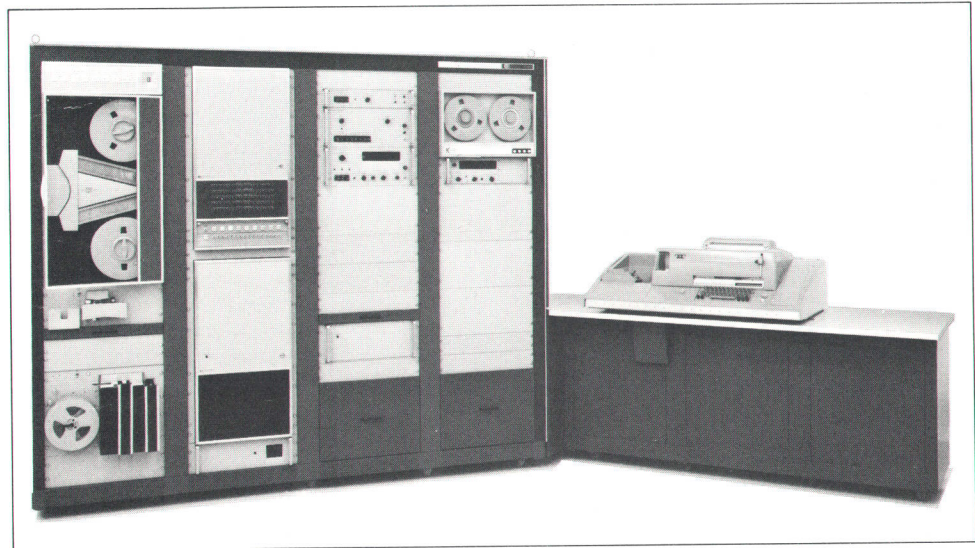
Fig. 5. Hughes Aircraft Company uses the HP Model 7389 for testing missile subassemblies. It reduces test times to 15 seconds from 5 minutes per module.
