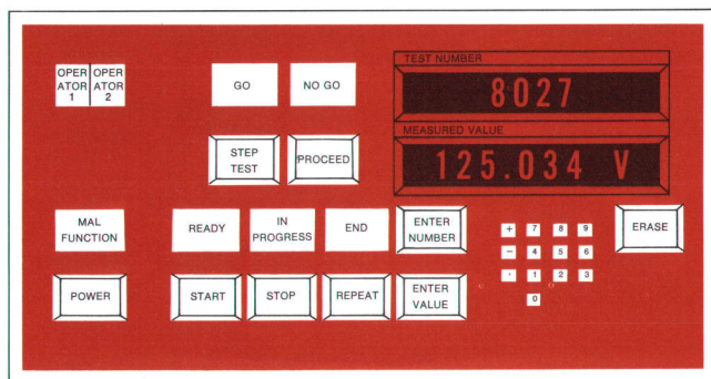
Fig. 3. One thing to consider when deciding on the form of a test system is how the operator will control the system. A teleprinter is a very versatile method which is used in most multipurpose systems. A control panel like this one is less versatile but easier to understand and more foolproof.
